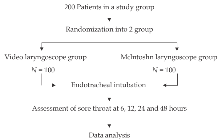
Fig. 1: Data-flow diagram
